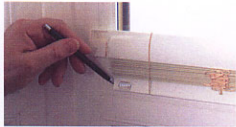
4. Using blind, mark positions for the cord grommet holes
